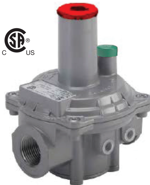
STANDARD MODEL
